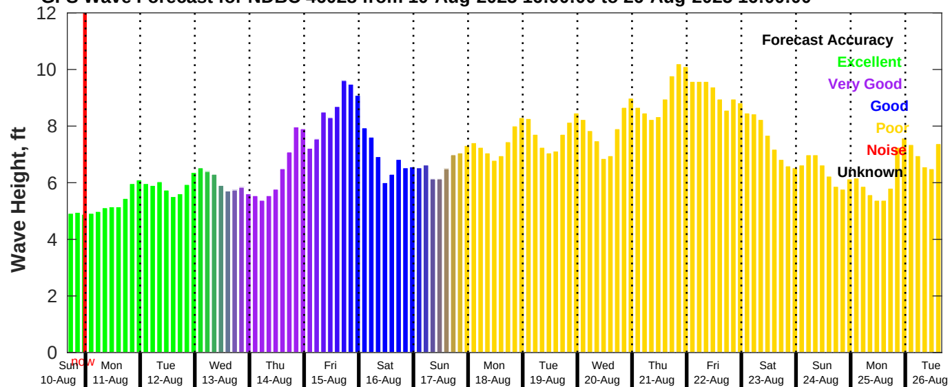
GFS Wave Forecast for NDBC 46028 from 10-Aug-2025 16:00:00 to 26-Aug-2025 16:00:00
