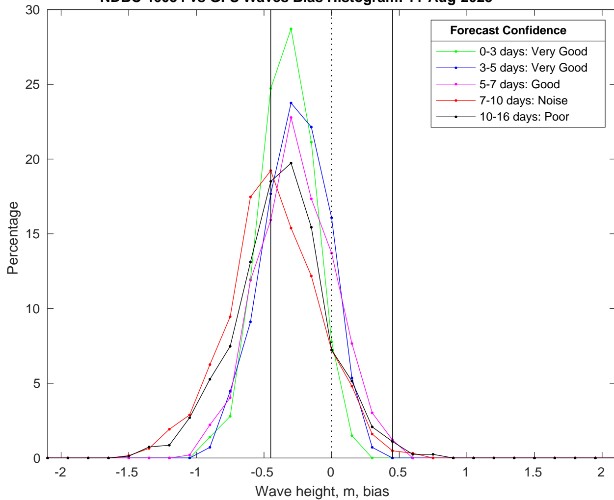
NDBC 46054 vs GFS Waves Bias Histogram: 11-Aug-2025
