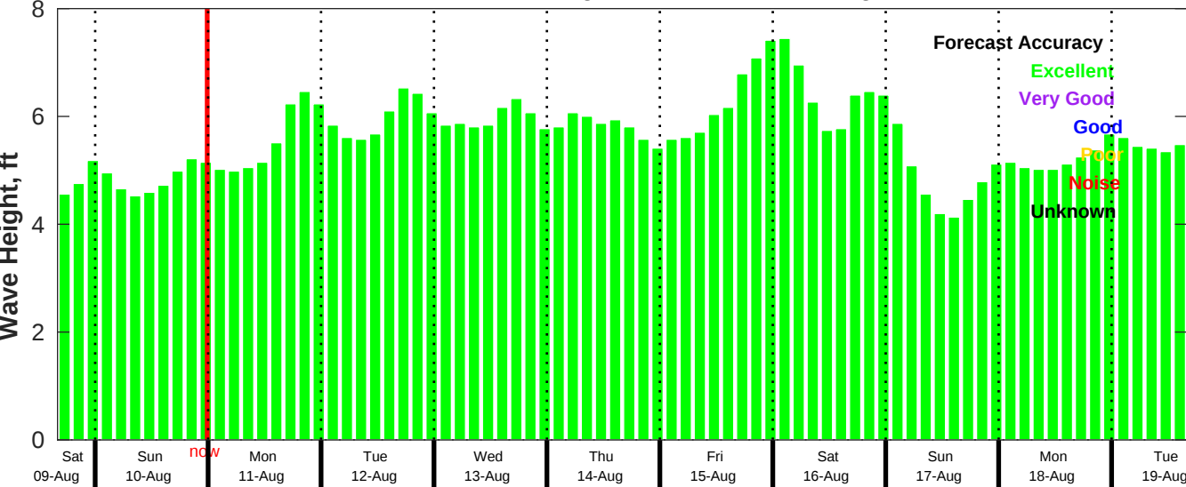
CMEMS Wave Forecast for NDBC 46054 from 09-Aug-2025 16:00:00 to 19-Aug-2025 16:00:00
