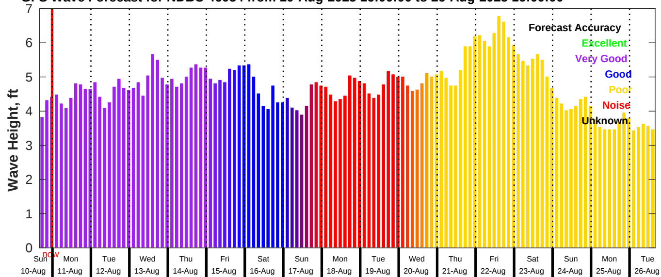
GFS Wave Forecast for NDBC 46054 from 10-Aug-2025 16:00:00 to 26-Aug-2025 16:00:00
