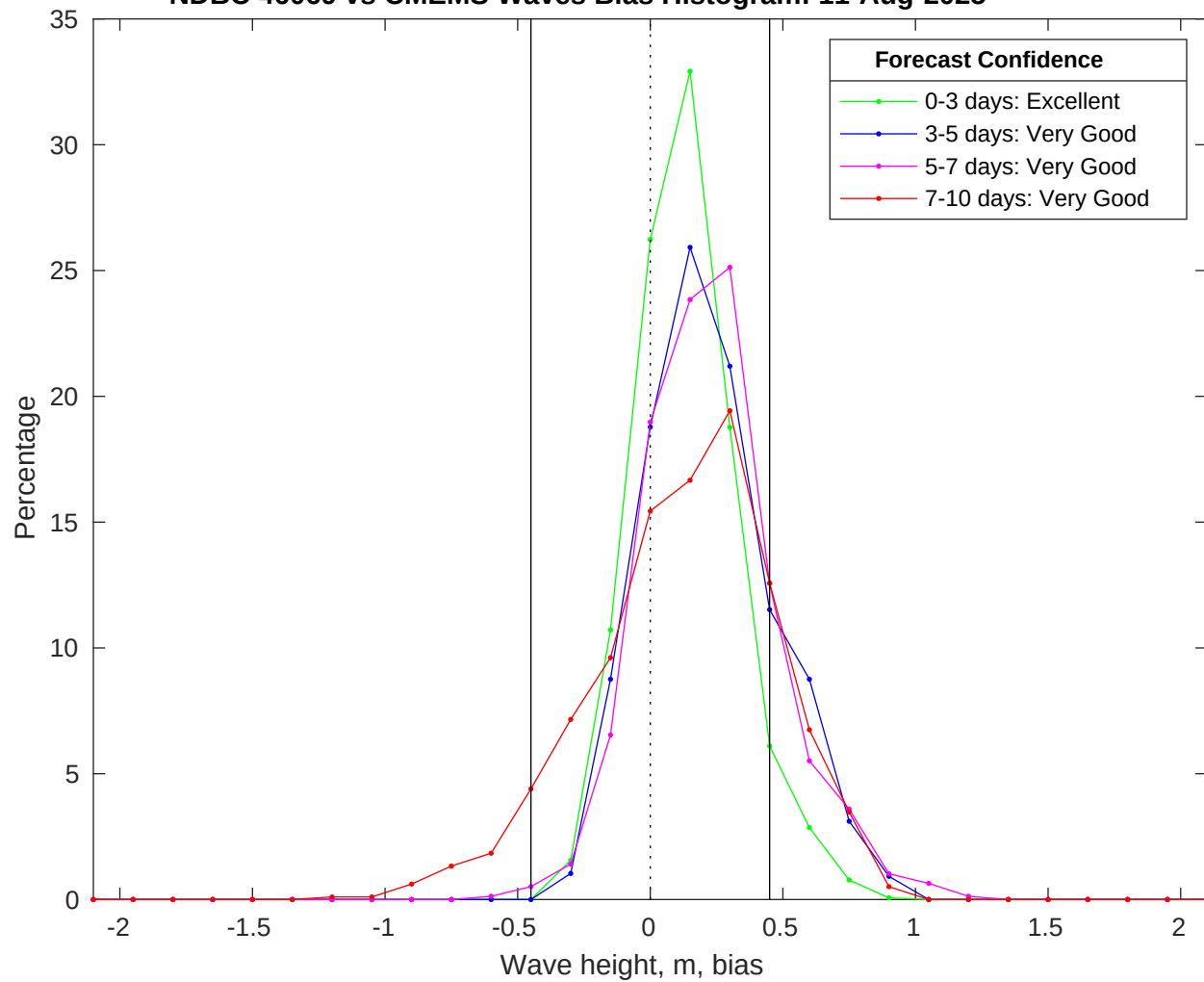
NDBC 46069 vs CMEMS Waves Bias Histogram: 11-Aug-2025
