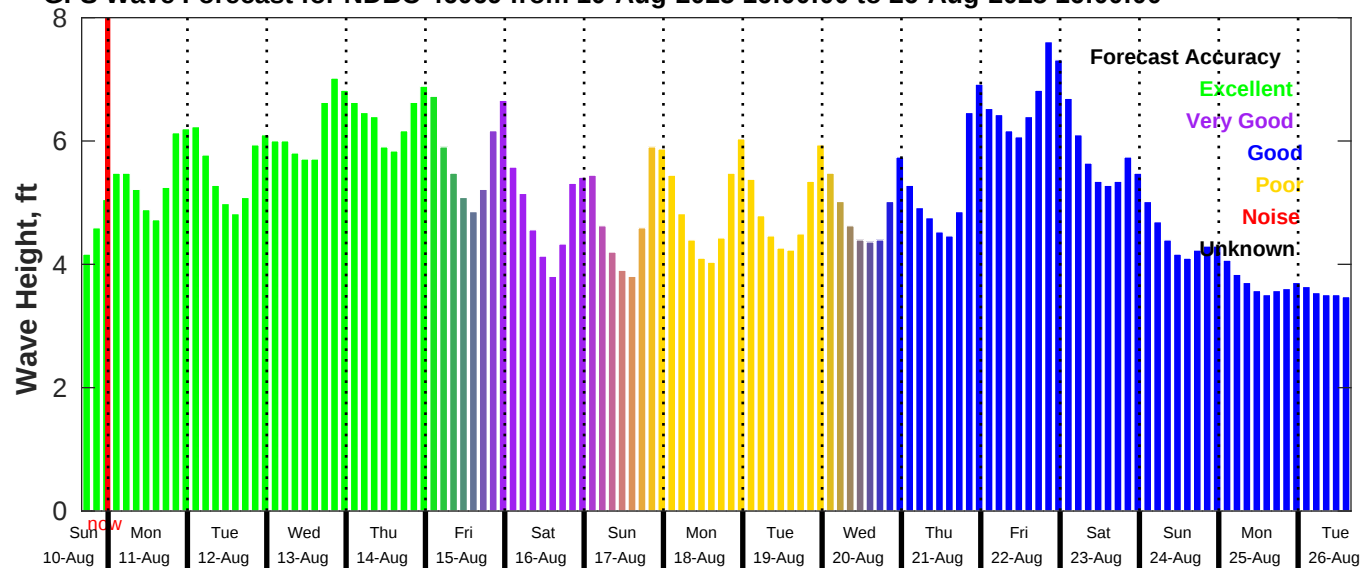
GFS Wave Forecast for NDBC 46069 from 10-Aug-2025 16:00:00 to 26-Aug-2025 16:00:00
