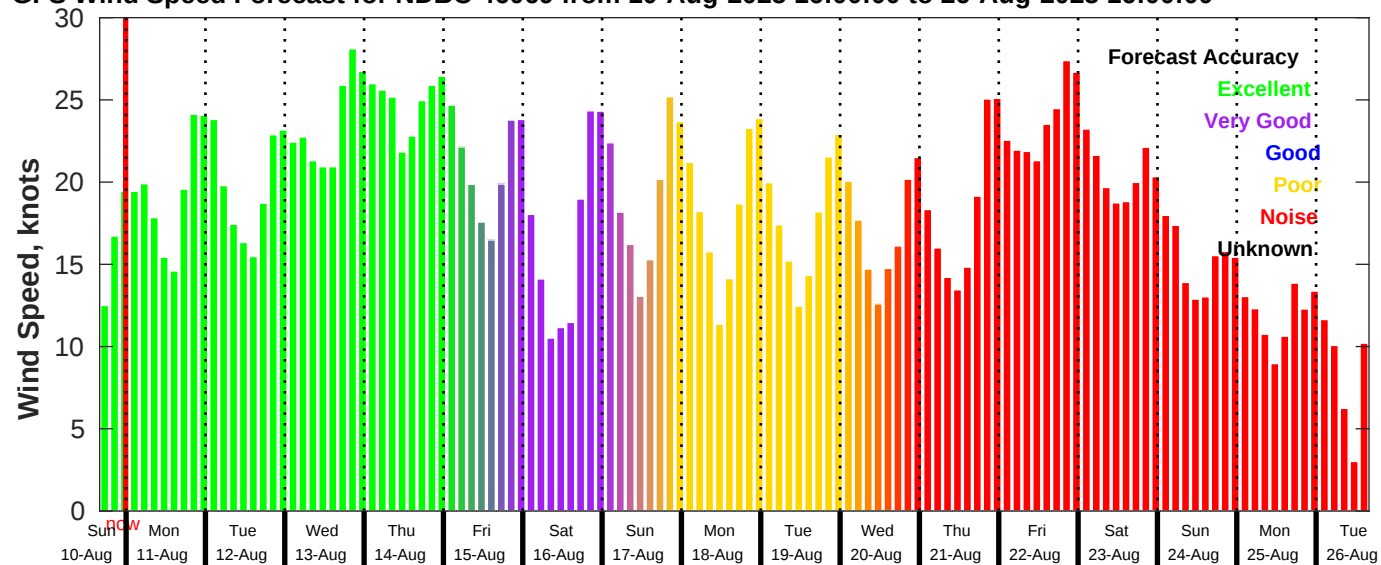
GFS Wind Speed Forecast for NDBC 46069 from 10-Aug-2025 16:00:00 to 26-Aug-2025 16:00:00
