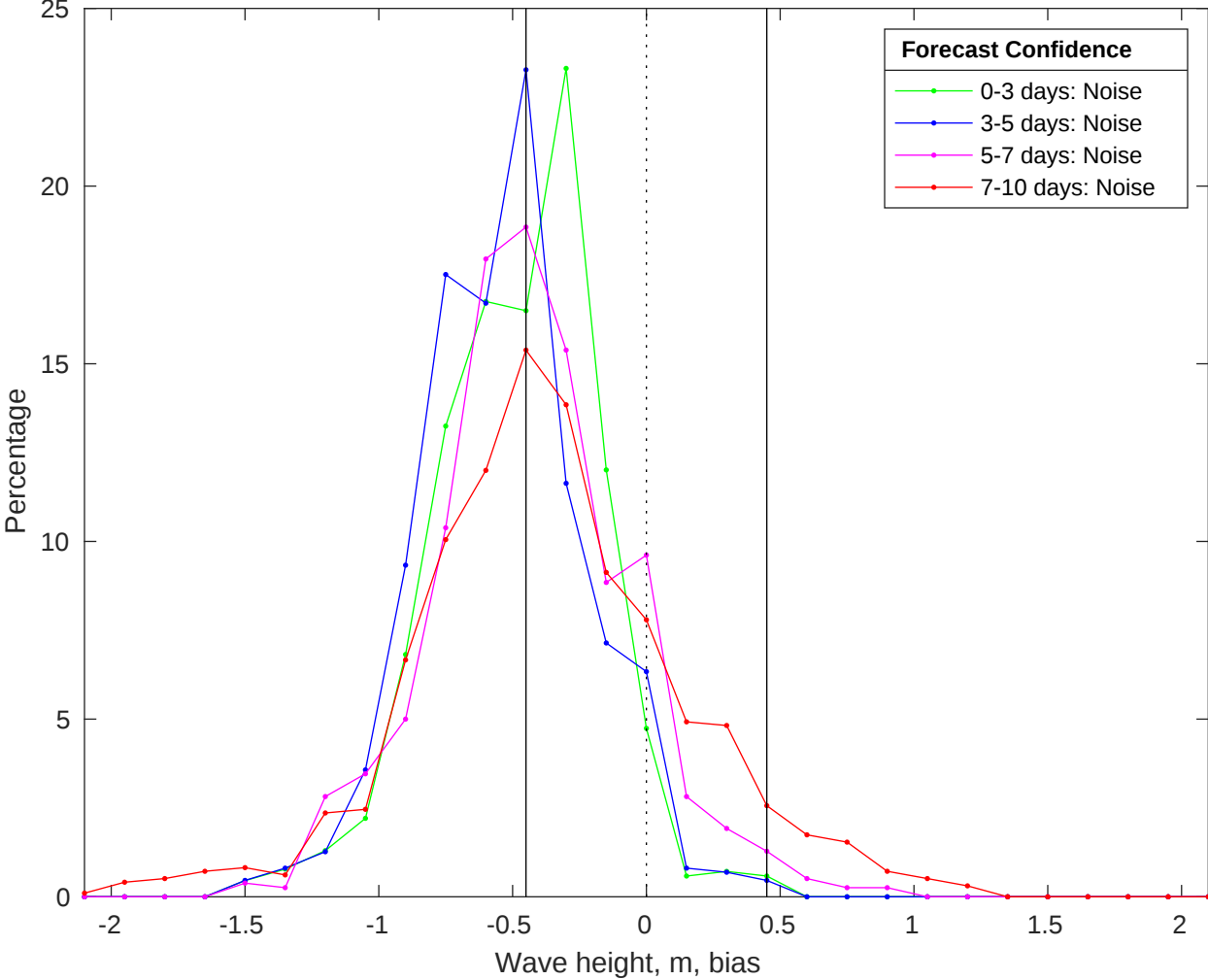
NDBC 51209 vs CMEMS Waves Bias Histogram: 11-Aug-2025
