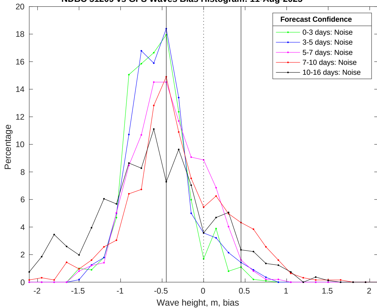
NDBC 51209 vs GFS Waves Bias Histogram: 11-Aug-2025
