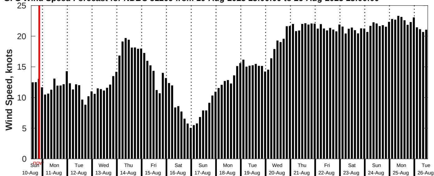
GFS Wind Speed Forecast for NDBC 51209 from 10-Aug-2025 13:00:00 to 26-Aug-2025 13:00:00
