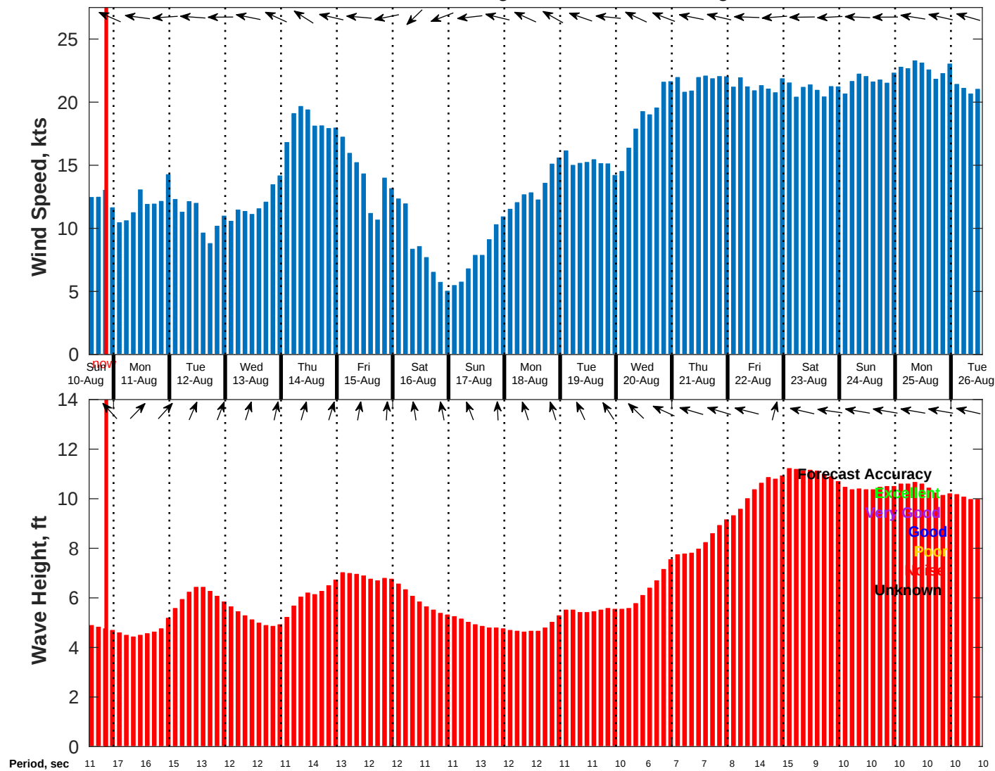
Wind & Wave Forecast for NDBC 51209 from 10-Aug-2025 13:00:00 to 26-Aug-2025 13:00:00
