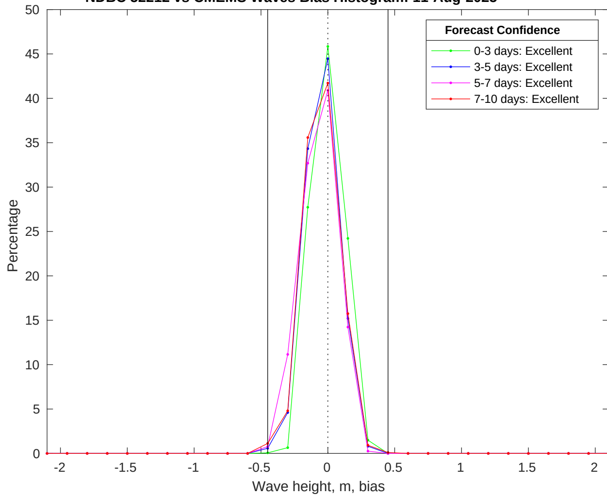
NDBC 52212 vs CMEMS Waves Bias Histogram: 11-Aug-2025
