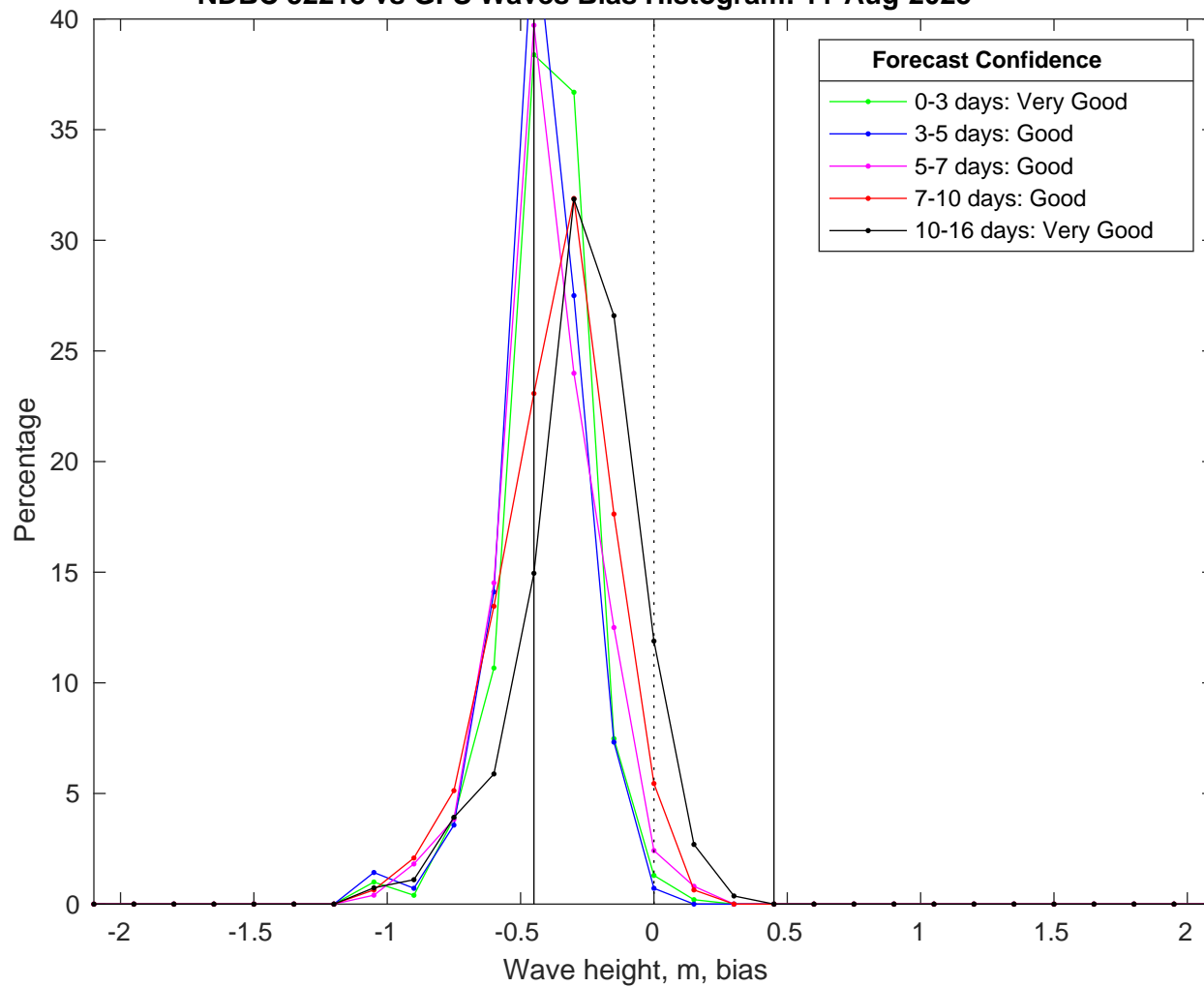
NDBC 52213 vs GFS Waves Bias Histogram: 11-Aug-2025
