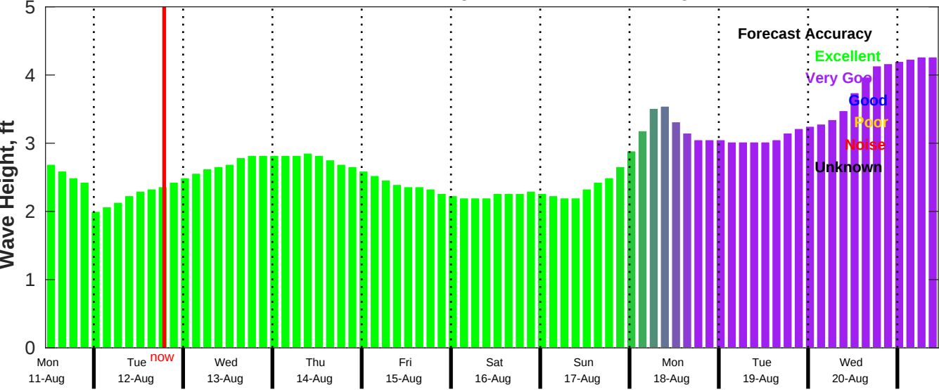
CMEMS Wave Forecast for NDBC 52213 from 10-Aug-2025 11:00:00 to 20-Aug-2025 11:00:00
