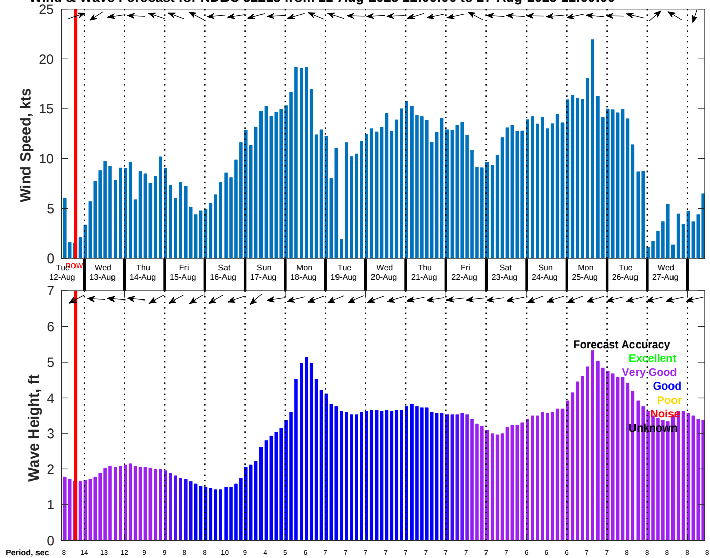
Wind & Wave Forecast for NDBC 52213 from 11-Aug-2025 11:00:00 to 27-Aug-2025 11:00:00
