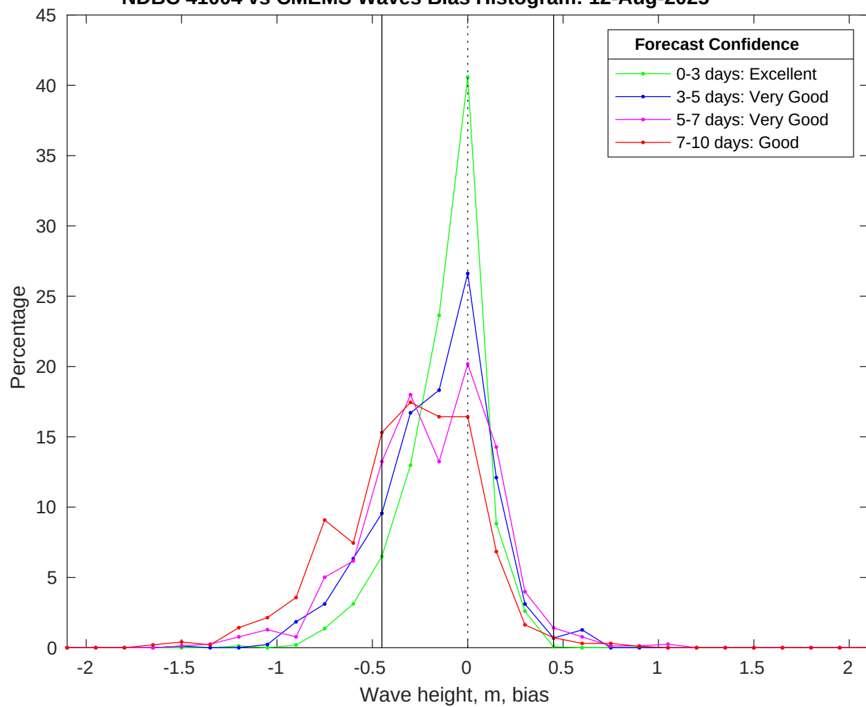
NDBC 41004 vs CMEMS Waves Bias Histogram: 12-Aug-2025
