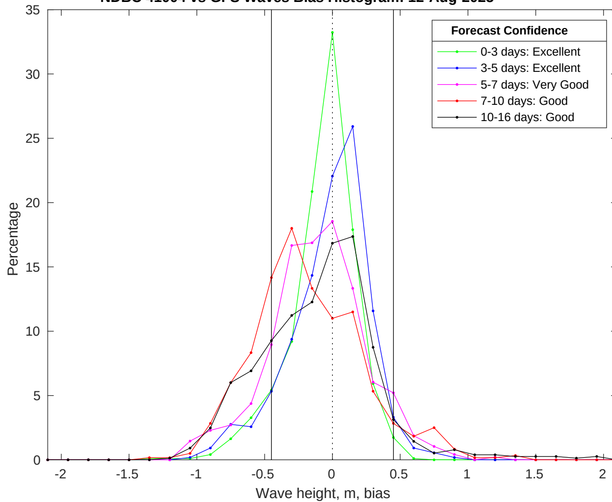
NDBC 41004 vs GFS Waves Bias Histogram: 12-Aug-2025
