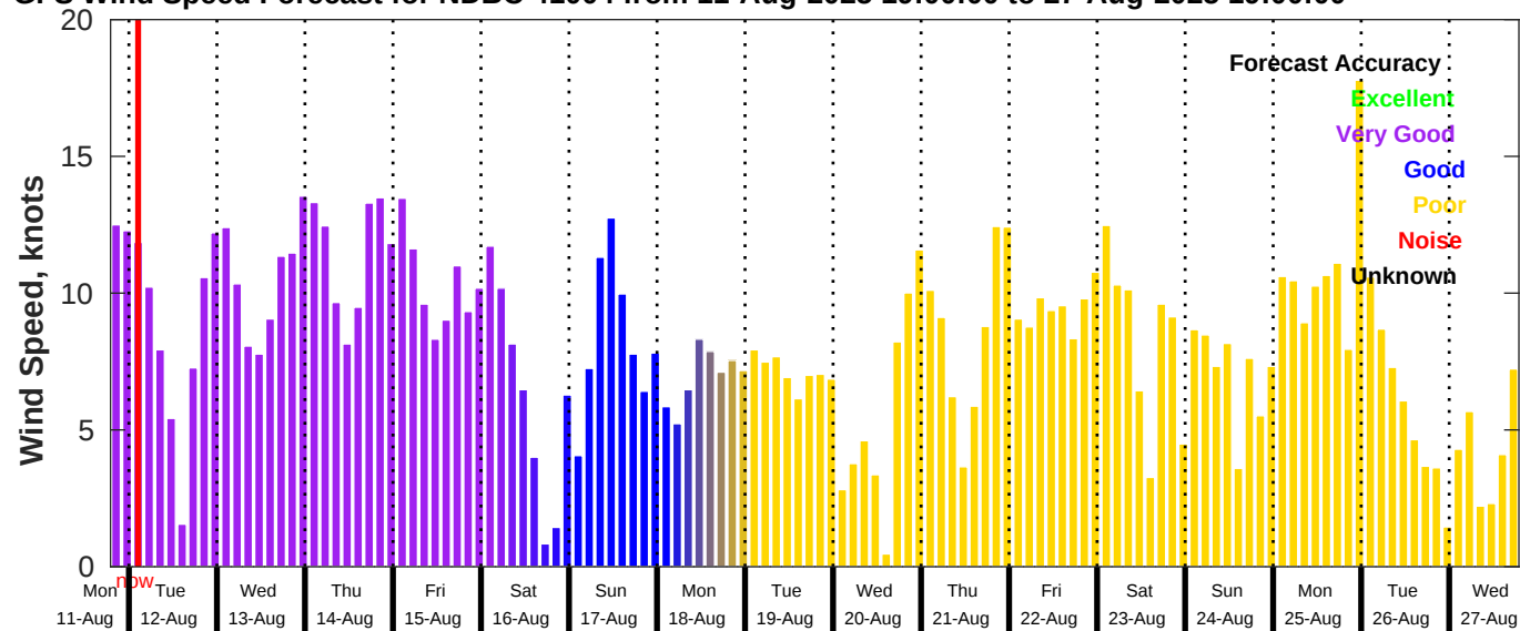
GFS Wind Speed Forecast for NDBC 41004 from 11-Aug-2025 19:00:00 to 27-Aug-2025 19:00:00
