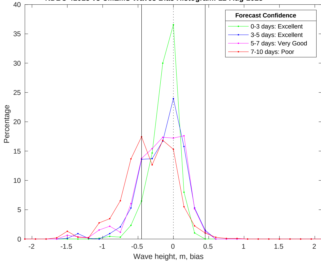
NDBC 41013 vs CMEMS Waves Bias Histogram: 12-Aug-2025
