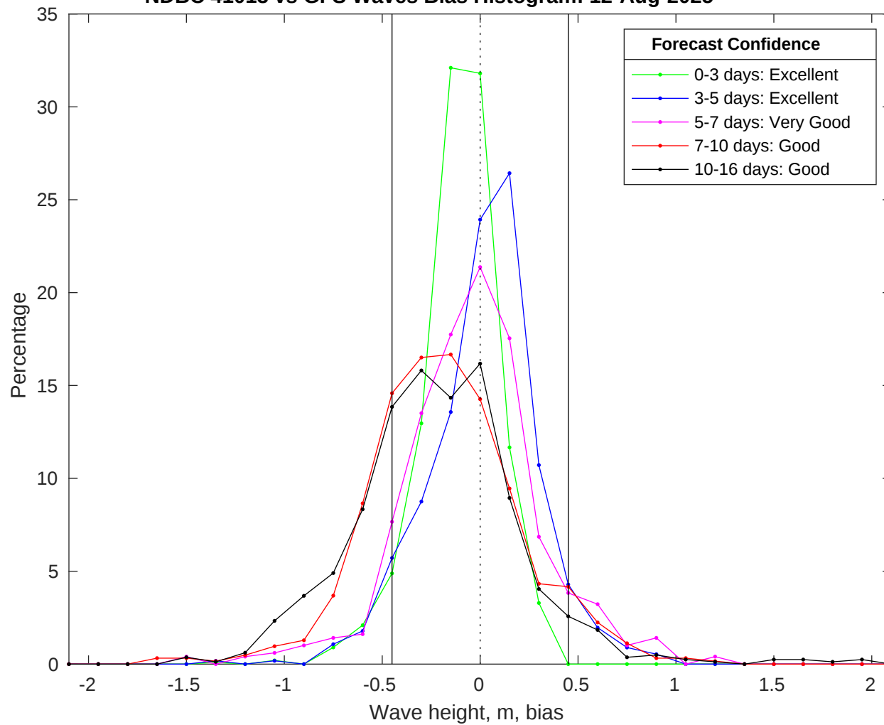
NDBC 41013 vs GFS Waves Bias Histogram: 12-Aug-2025
