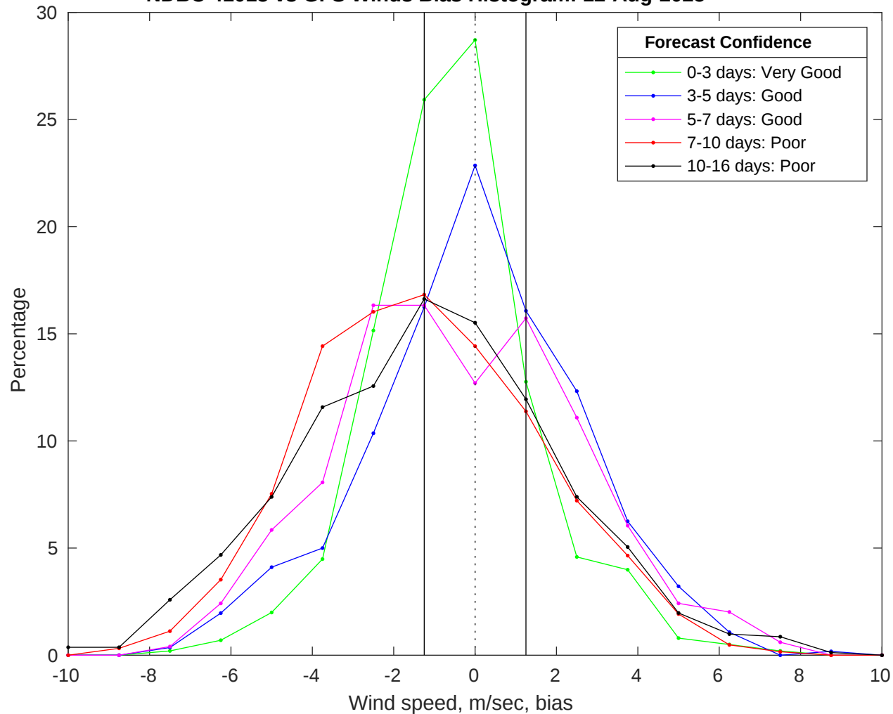
NDBC 41013 vs GFS Winds Bias Histogram: 12-Aug-2025
