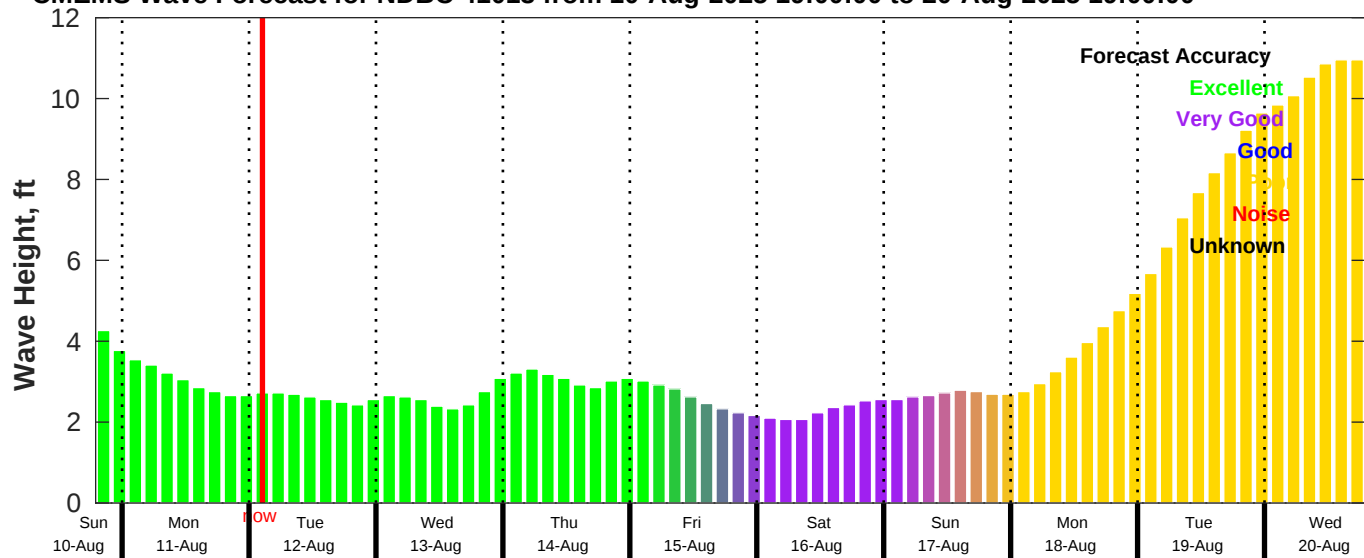
CMEMS Wave Forecast for NDBC 41013 from 10-Aug-2025 19:00:00 to 20-Aug-2025 19:00:00
