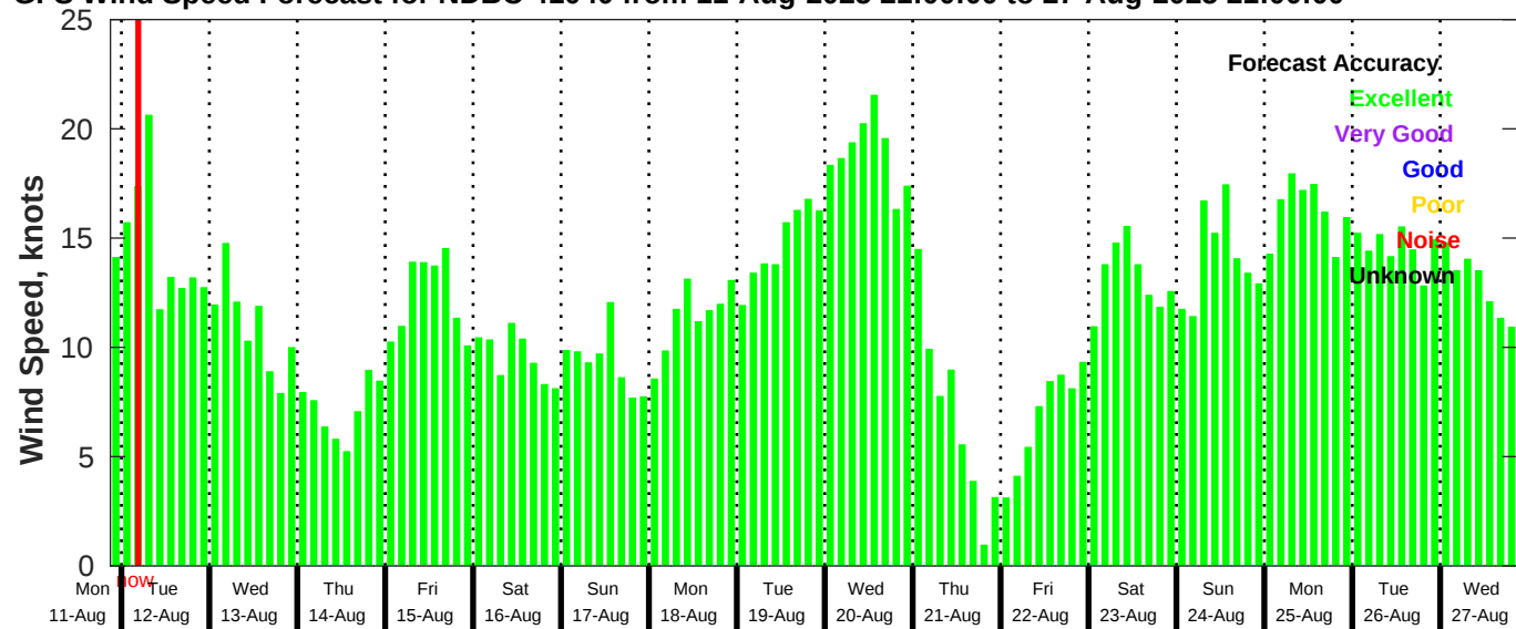
GFS Wind Speed Forecast for NDBC 41040 from 11-Aug-2025 21:00:00 to 27-Aug-2025 21:00:00
