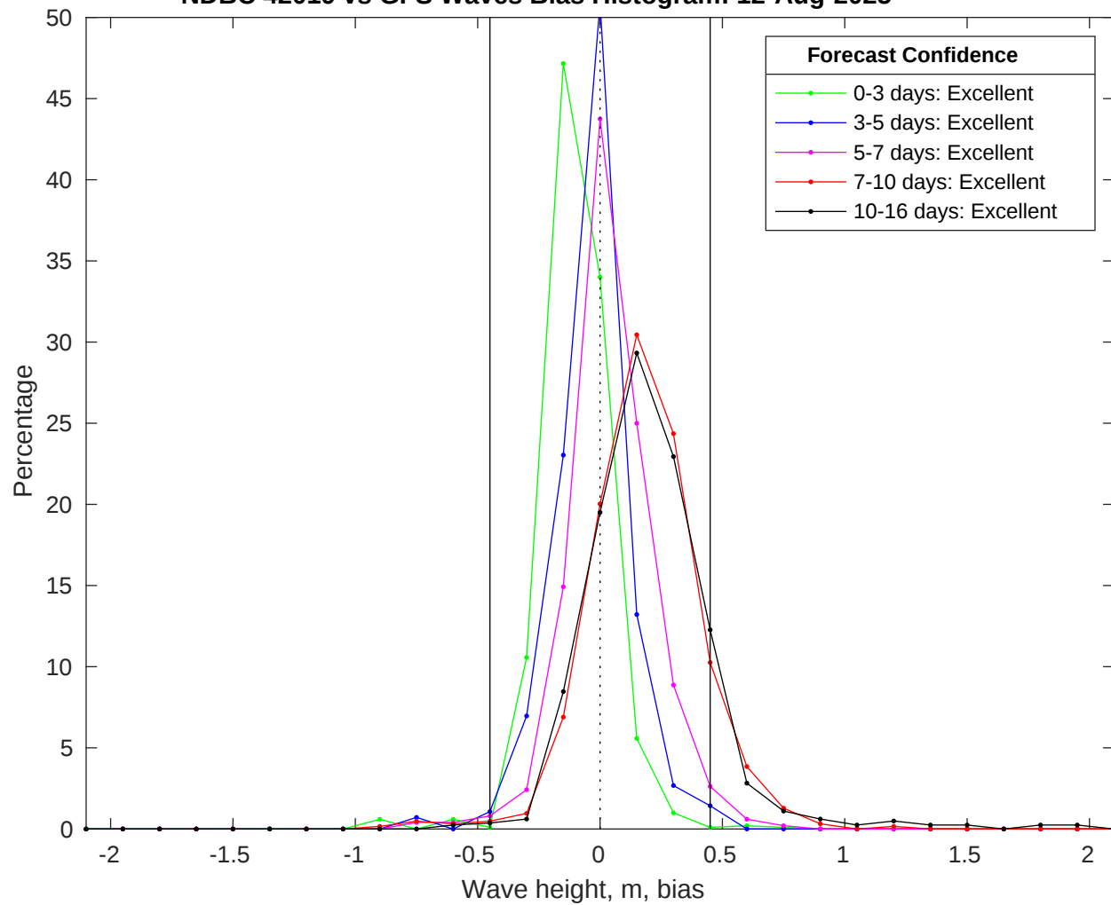
NDBC 42019 vs GFS Waves Bias Histogram: 12-Aug-2025
