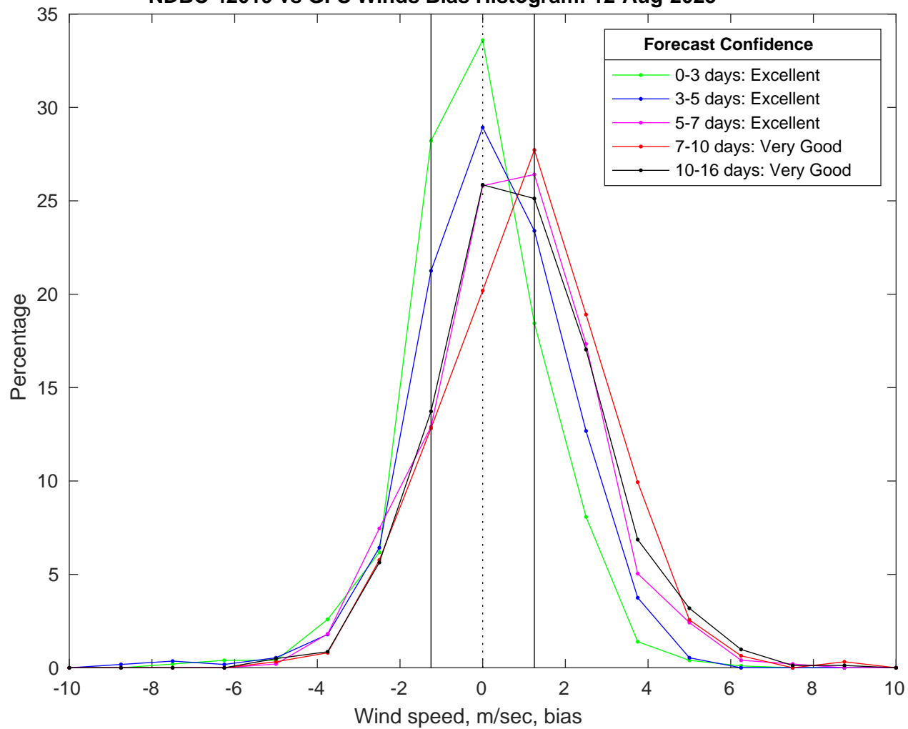
NDBC 42019 vs GFS Winds Bias Histogram: 12-Aug-2025
