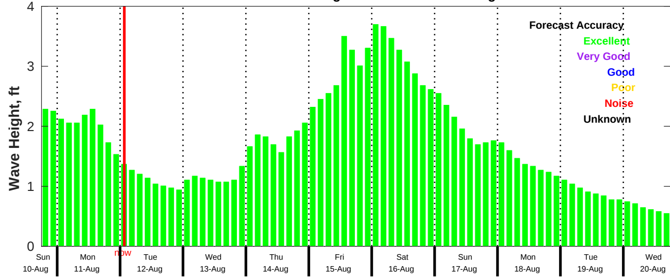
CMEMS Wave Forecast for NDBC 42019 from 10-Aug-2025 18:00:00 to 20-Aug-2025 18:00:00
