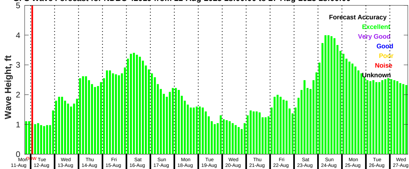
GFS Wave Forecast for NDBC 42019 from 11-Aug-2025 18:00:00 to 27-Aug-2025 18:00:00
