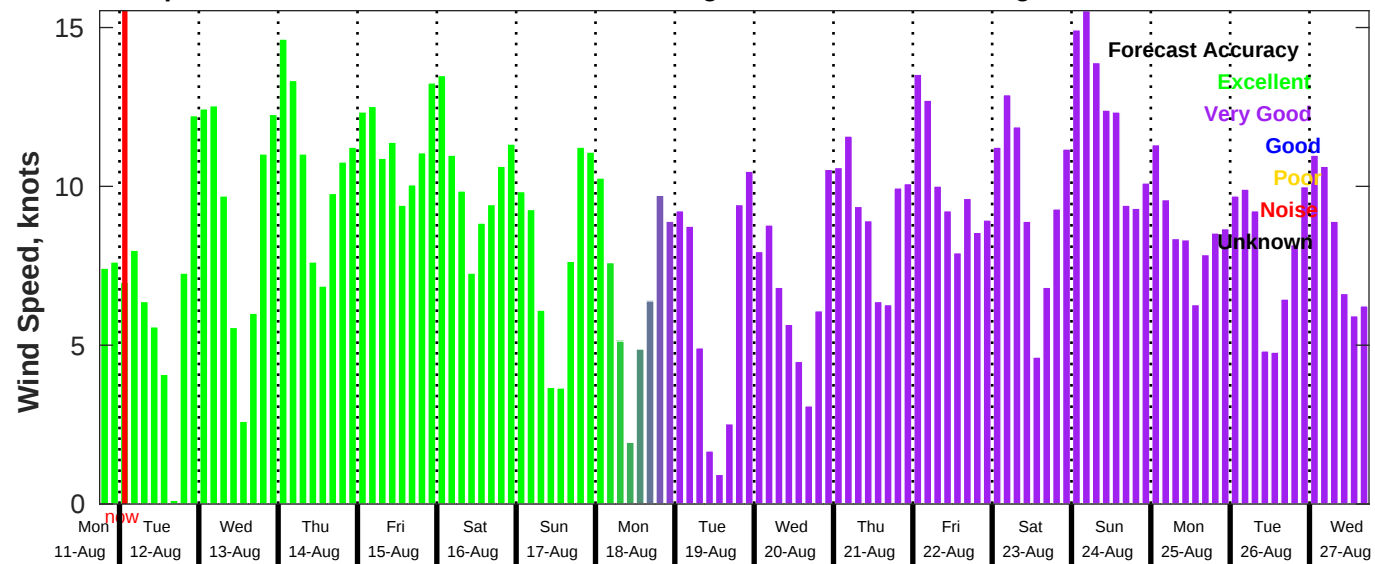
GFS Wind Speed Forecast for NDBC 42019 from 11-Aug-2025 18:00:00 to 27-Aug-2025 18:00:00
