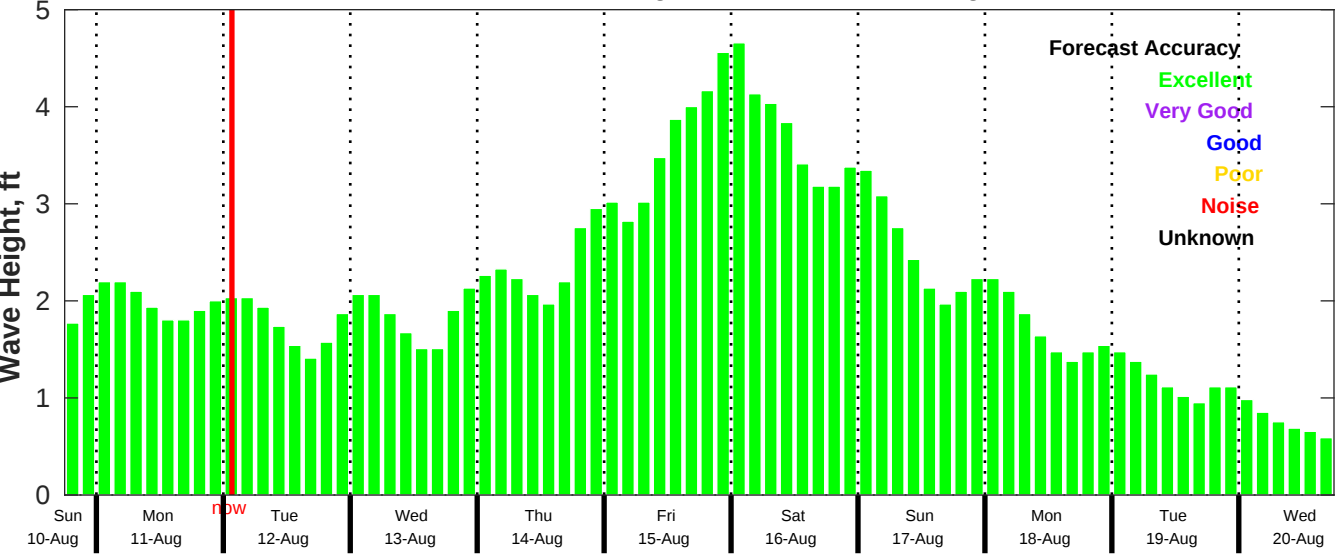
CMEMS Wave Forecast for NDBC 42020 from 10-Aug-2025 18:00:00 to 20-Aug-2025 18:00:00
