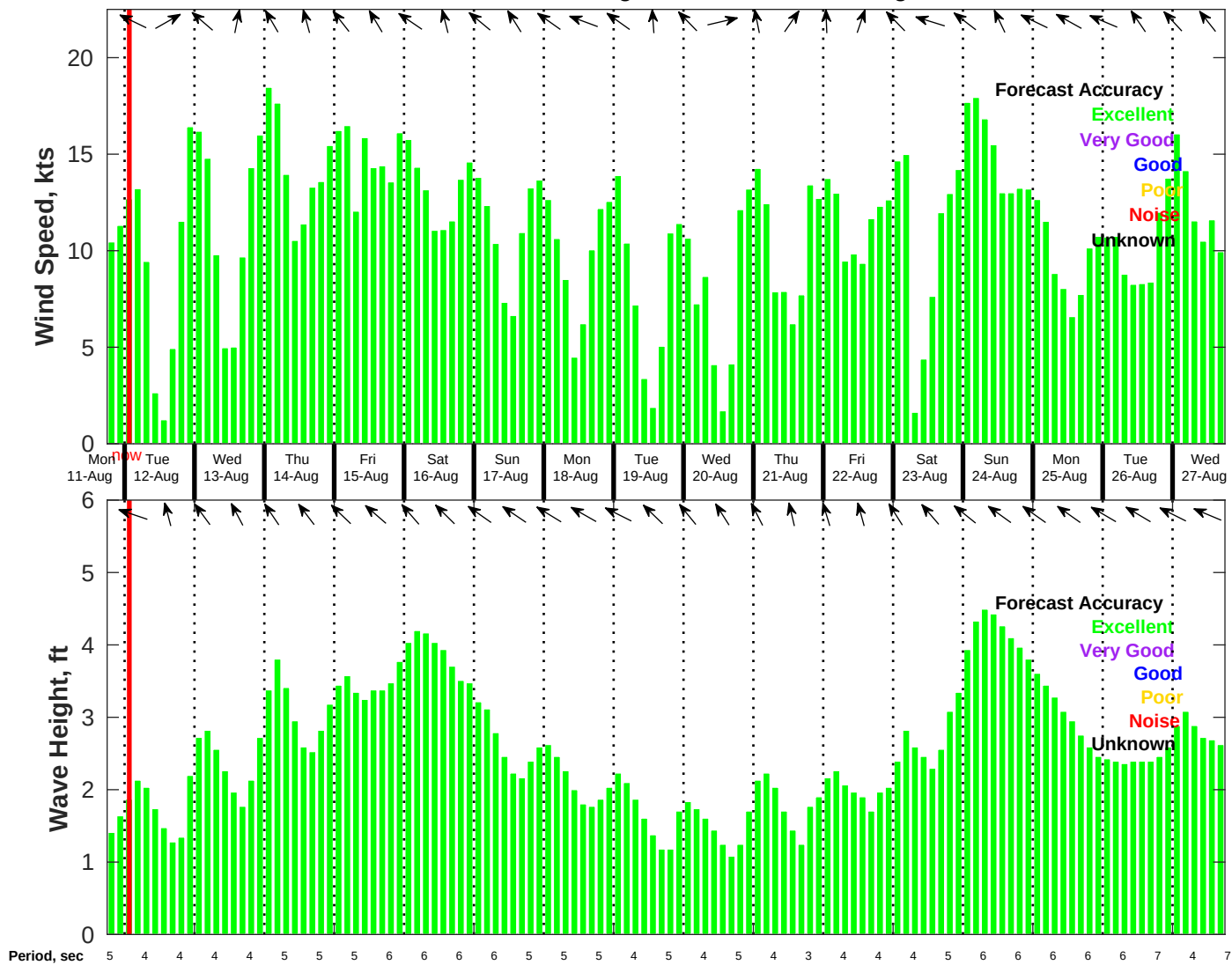
Wind & Wave Forecast for NDBC 42020 from 11-Aug-2025 18:00:00 to 27-Aug-2025 18:00:00
