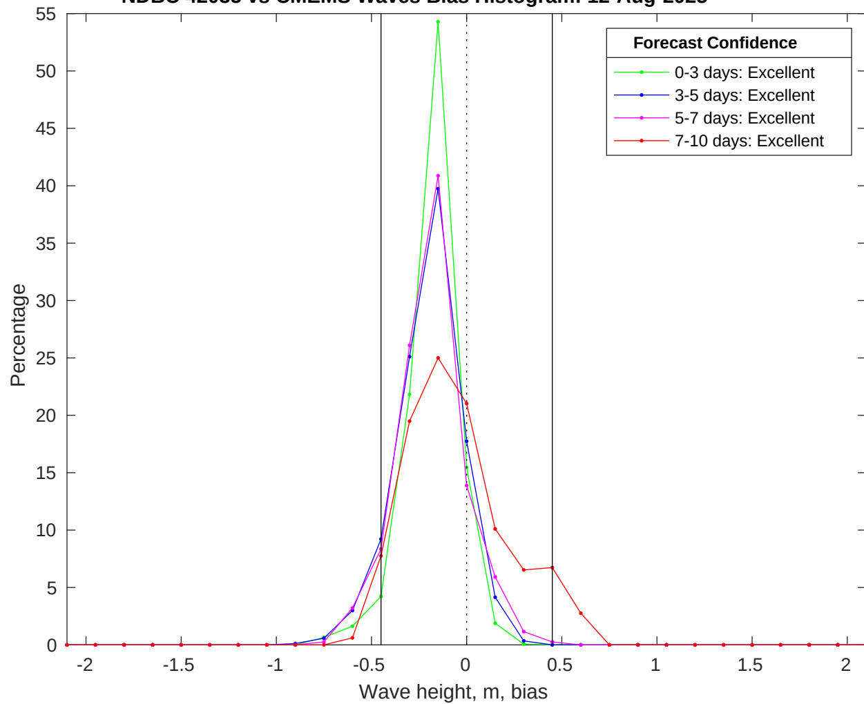
NDBC 42035 vs CMEMS Waves Bias Histogram: 12-Aug-2025
