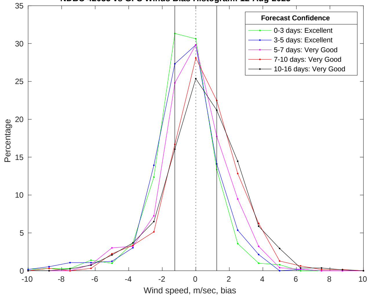
NDBC 42035 vs GFS Winds Bias Histogram: 12-Aug-2025
