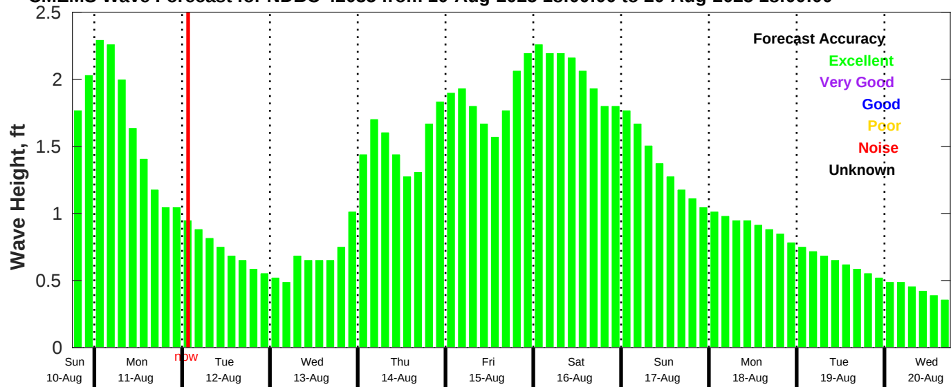
CMEMS Wave Forecast for NDBC 42035 from 10-Aug-2025 18:00:00 to 20-Aug-2025 18:00:00
