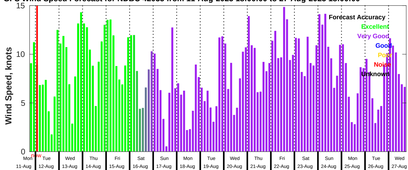
GFS Wind Speed Forecast for NDBC 42035 from 11-Aug-2025 18:00:00 to 27-Aug-2025 18:00:00
