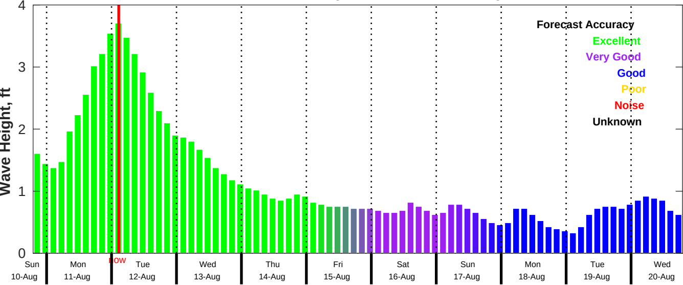
CMEMS Wave Forecast for NDBC 42036 from 10-Aug-2025 19:00:00 to 20-Aug-2025 19:00:00
