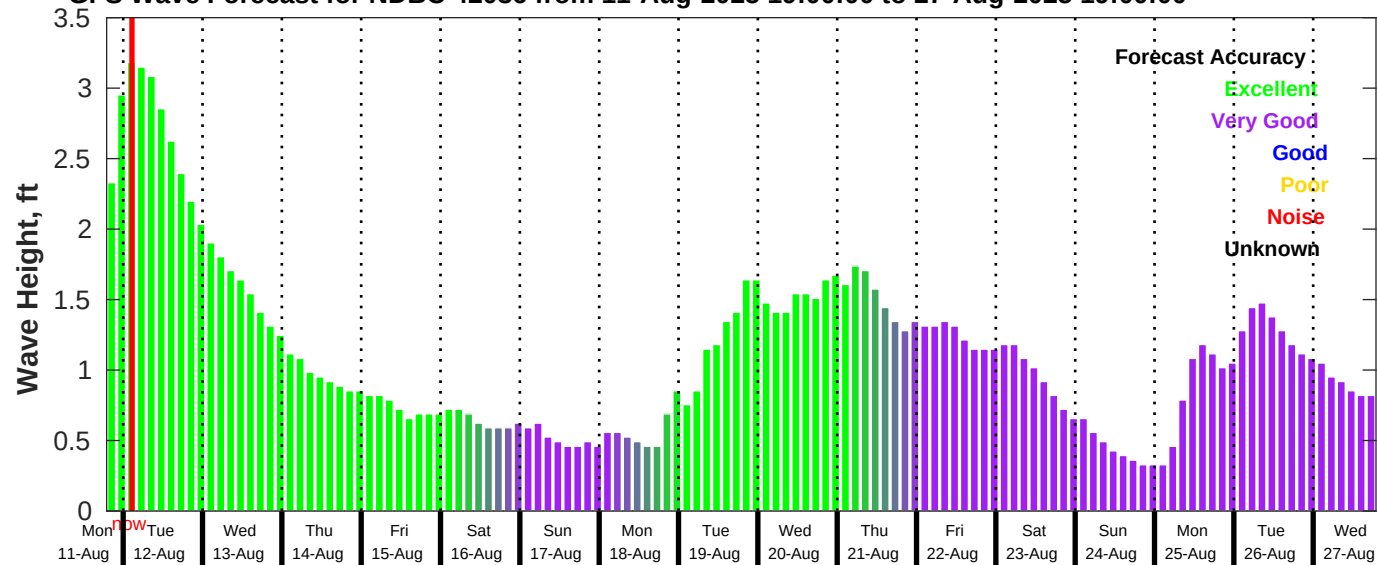
GFS Wave Forecast for NDBC 42036 from 11-Aug-2025 19:00:00 to 27-Aug-2025 19:00:00
