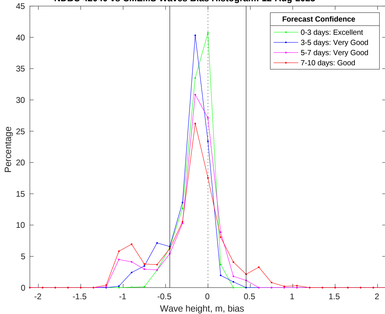
NDBC 42040 vs CMEMS Waves Bias Histogram: 12-Aug-2025
