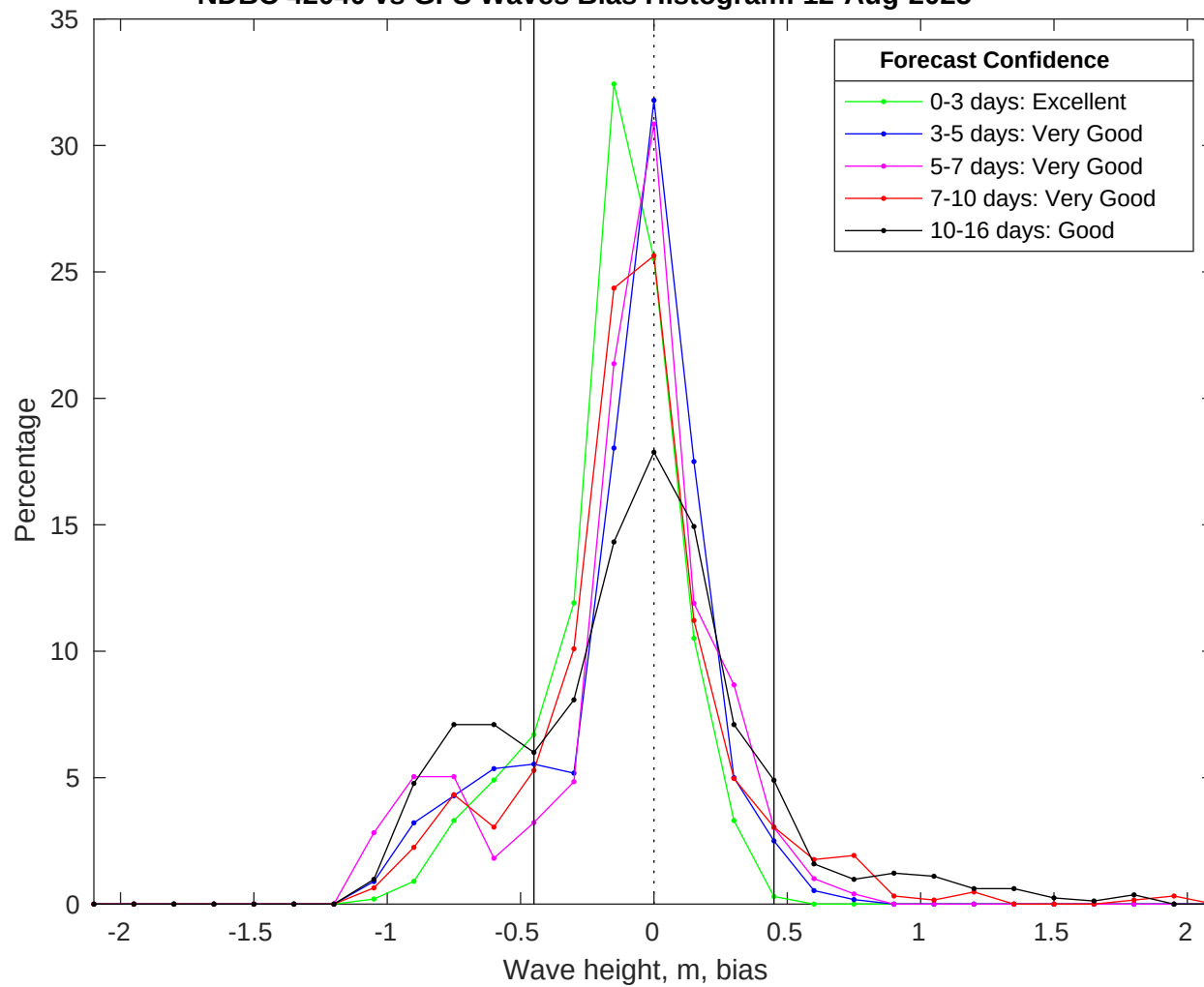
NDBC 42040 vs GFS Waves Bias Histogram: 12-Aug-2025
