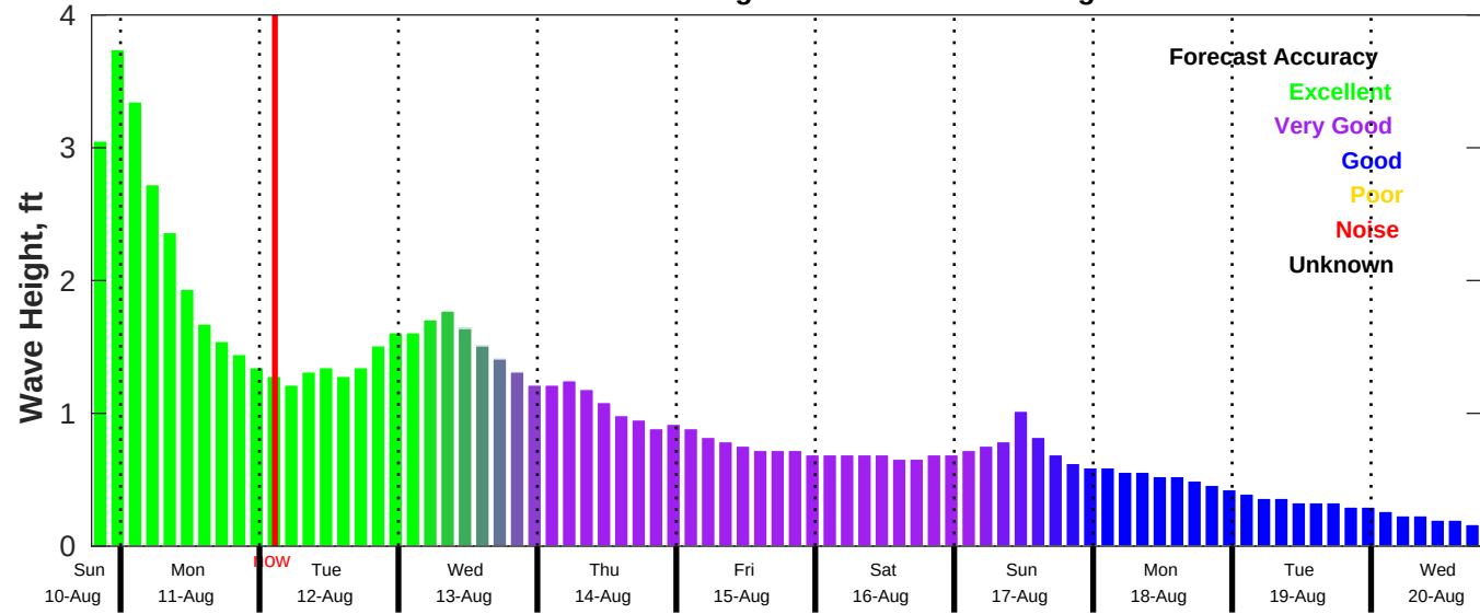
CMEMS Wave Forecast for NDBC 42040 from 10-Aug-2025 19:00:00 to 20-Aug-2025 19:00:00
