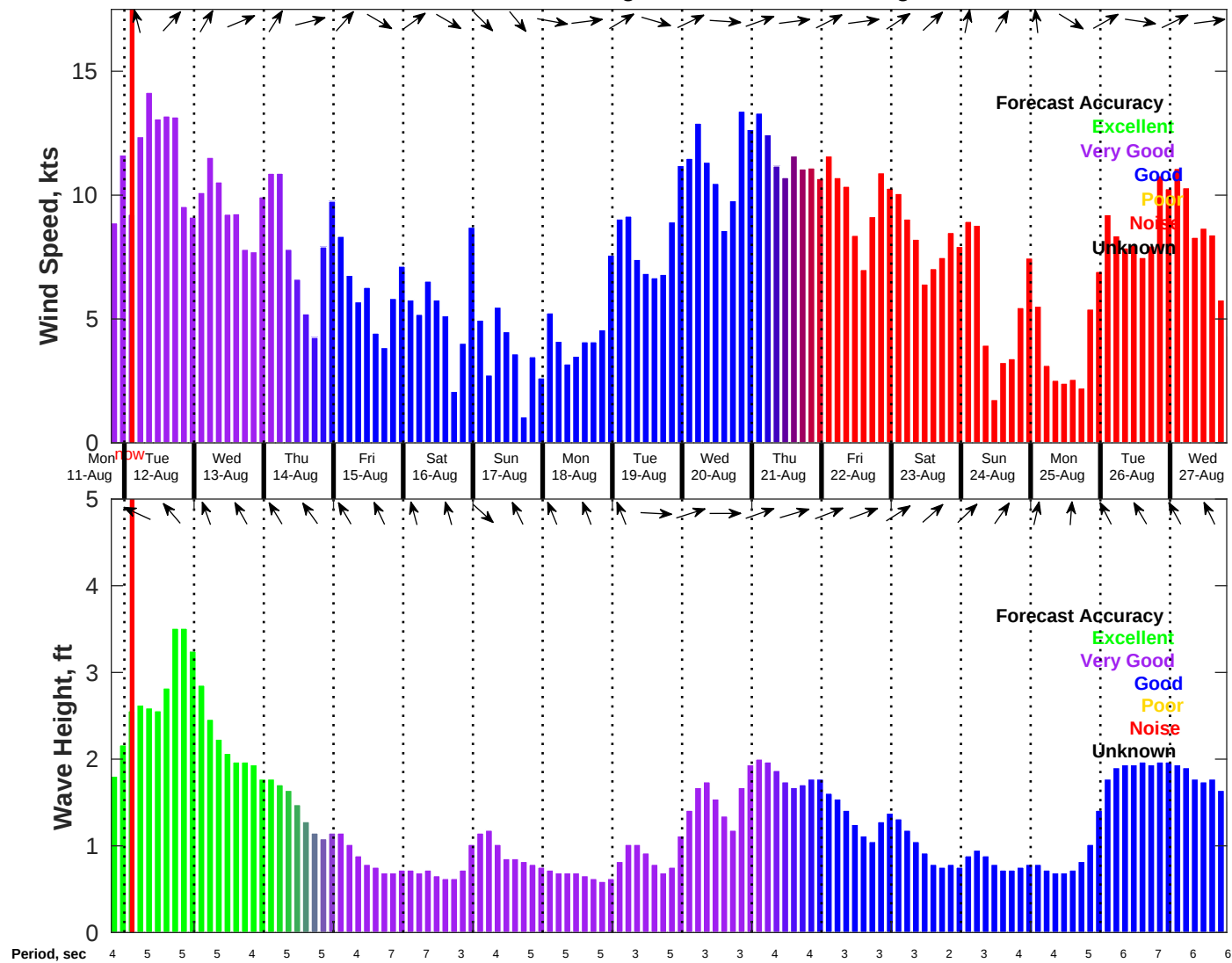
Wind & Wave Forecast for NDBC 42040 from 11-Aug-2025 19:00:00 to 27-Aug-2025 19:00:00
