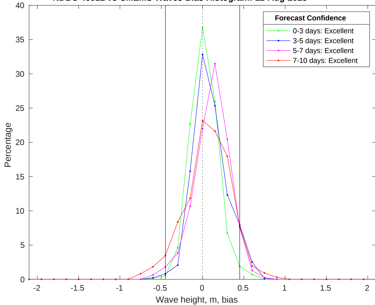
NDBC 46011 vs CMEMS Waves Bias Histogram: 12-Aug-2025
