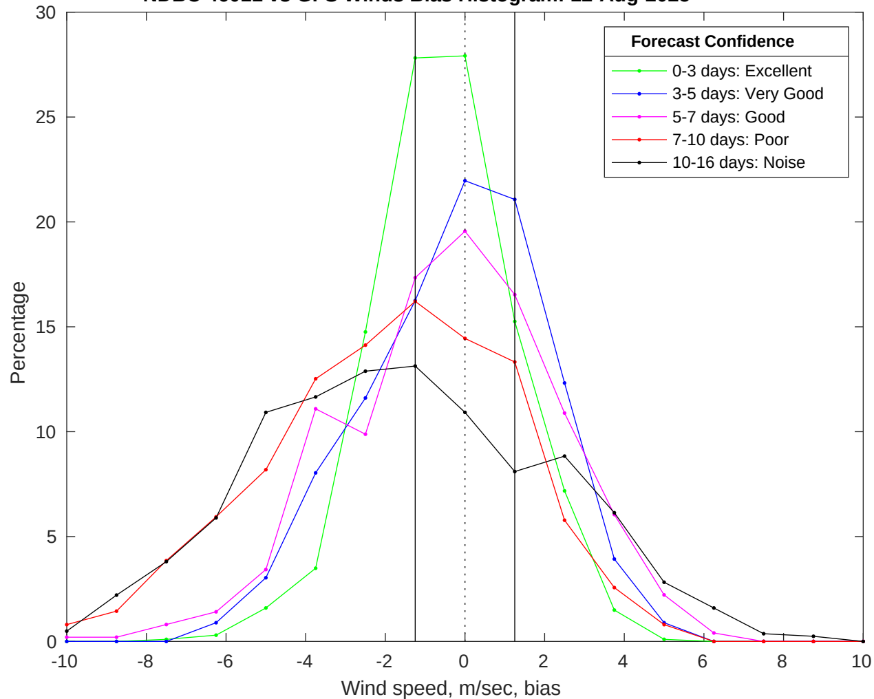
NDBC 46011 vs GFS Winds Bias Histogram: 12-Aug-2025
