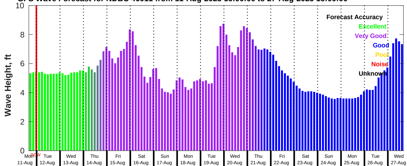
GFS Wave Forecast for NDBC 46011 from 11-Aug-2025 16:00:00 to 27-Aug-2025 16:00:00
