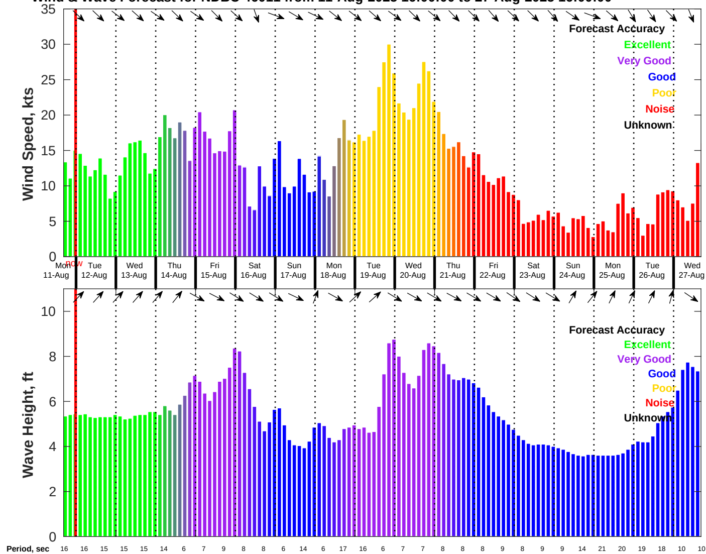
Wind & Wave Forecast for NDBC 46011 from 11-Aug-2025 16:00:00 to 27-Aug-2025 16:00:00
