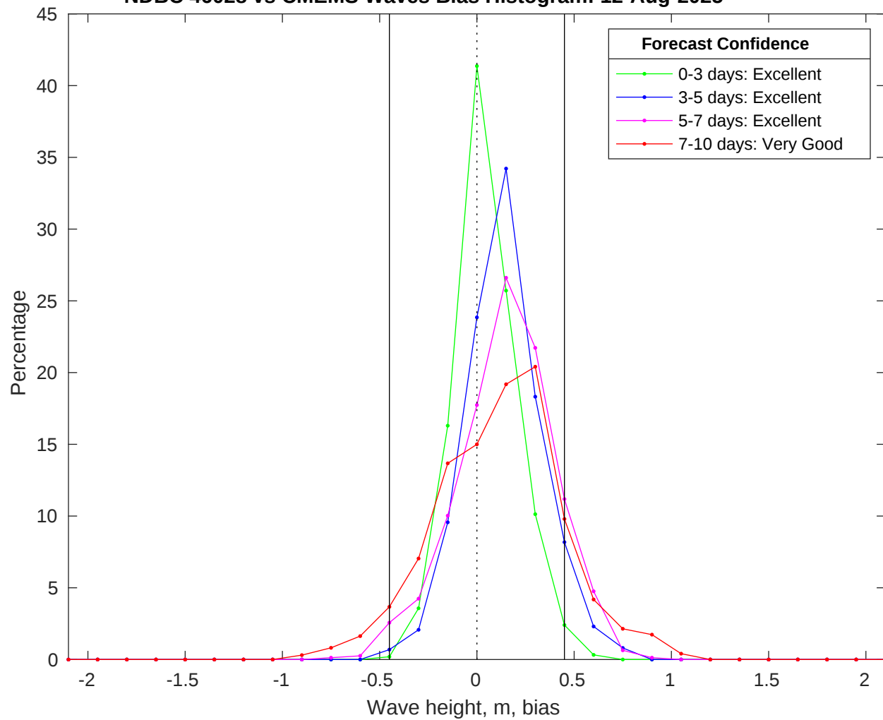
NDBC 46028 vs CMEMS Waves Bias Histogram: 12-Aug-2025
