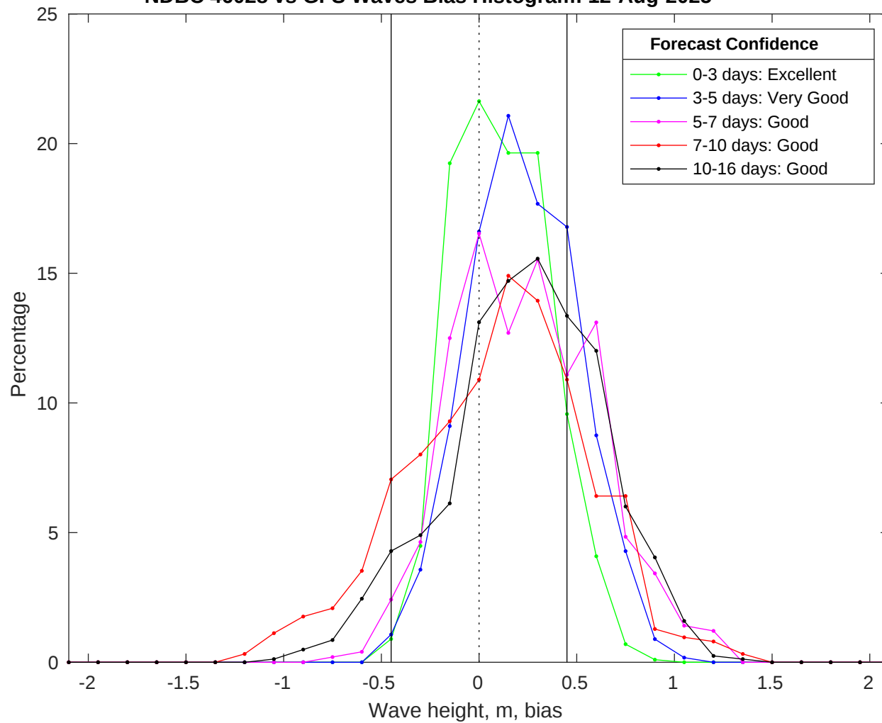
NDBC 46028 vs GFS Waves Bias Histogram: 12-Aug-2025
