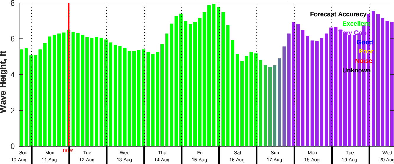
CMEMS Wave Forecast for NDBC 46028 from 10-Aug-2025 16:00:00 to 20-Aug-2025 16:00:00
