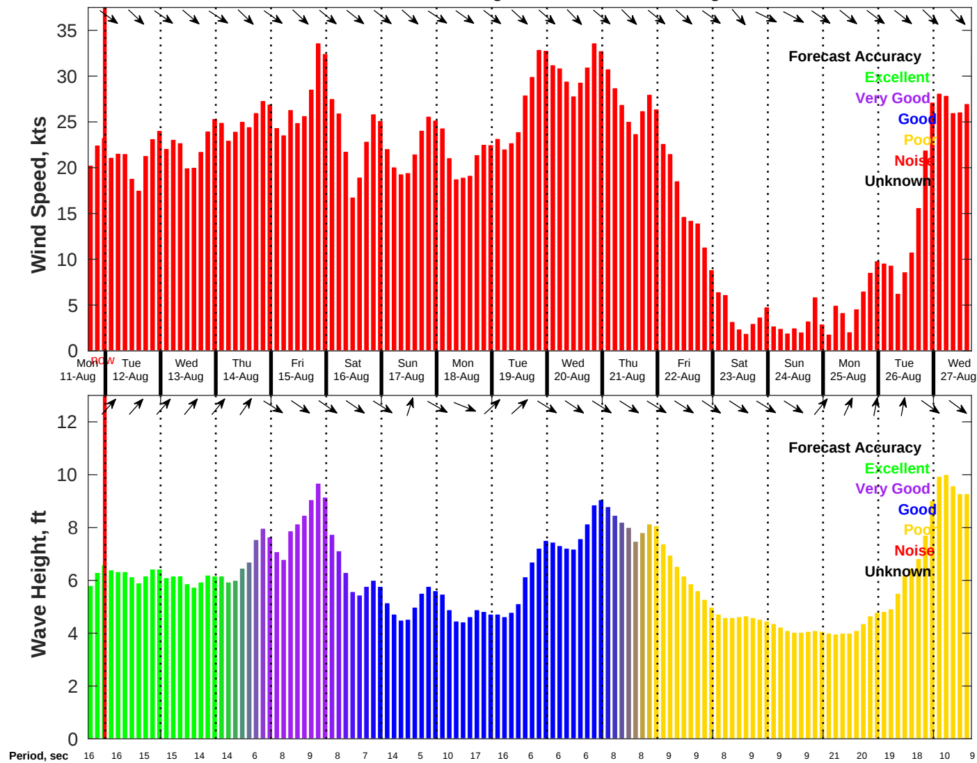
Wind & Wave Forecast for NDBC 46028 from 11-Aug-2025 16:00:00 to 27-Aug-2025 16:00:00
