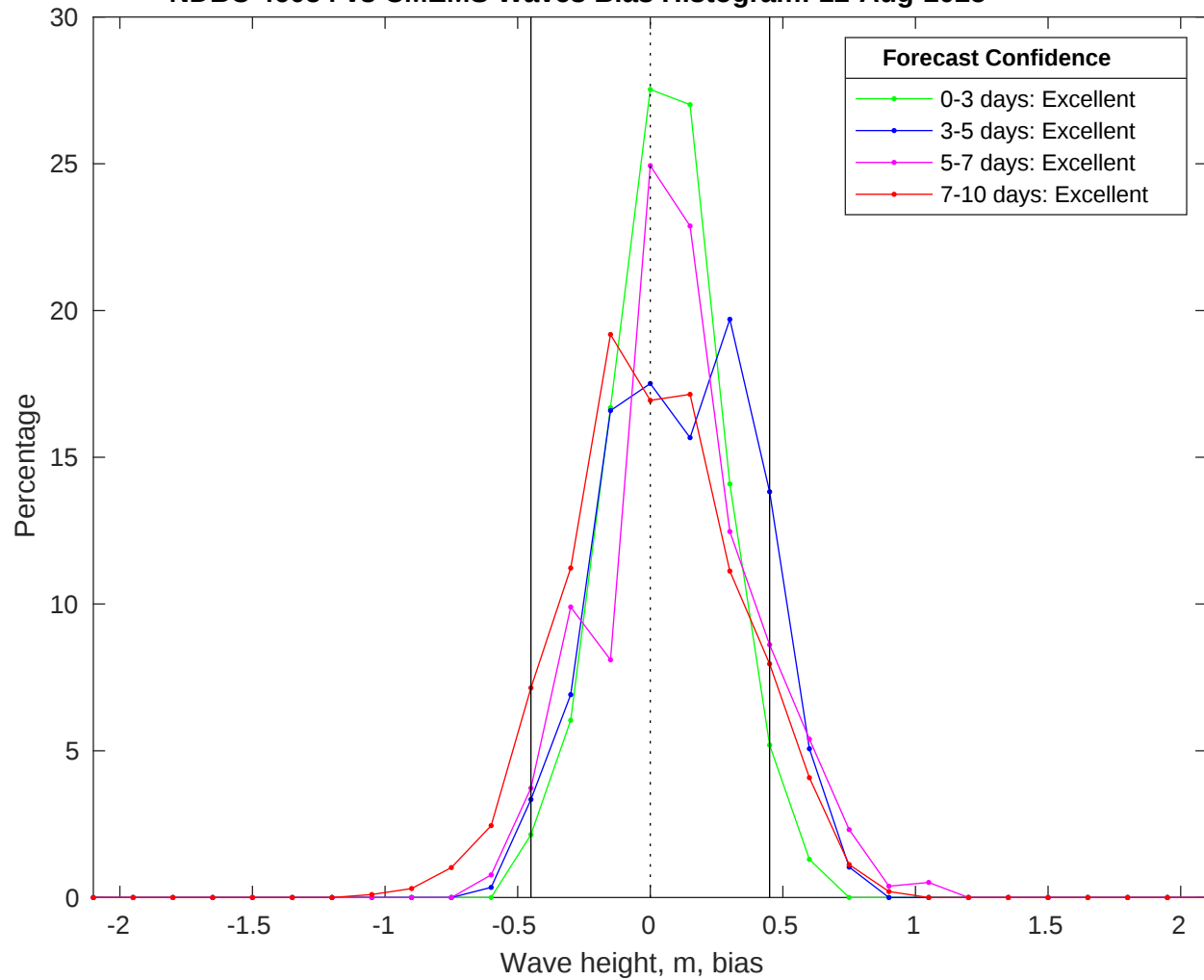
NDBC 46054 vs CMEMS Waves Bias Histogram: 12-Aug-2025
