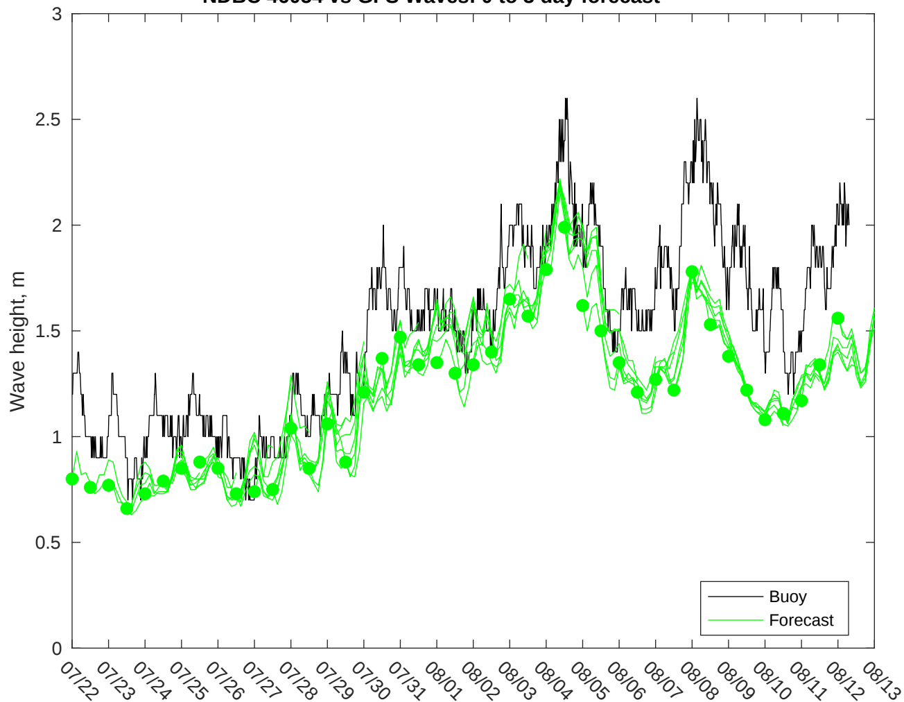
NDBC 46054 vs GFS Waves: 0 to 3 day forecast
